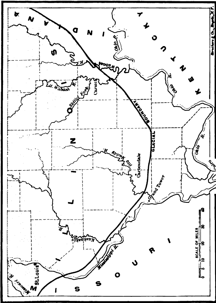
FIG. 47.—Glaciated region of southern Illinois.
